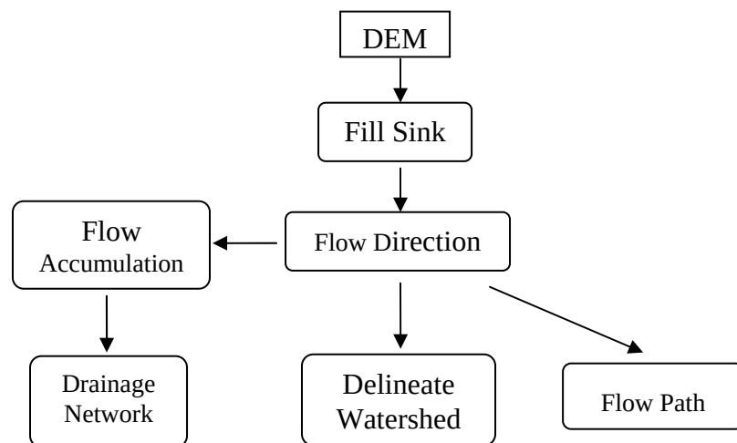
Figure2 Drainage Network Delineating Procedures described by Jenson and Domingue
