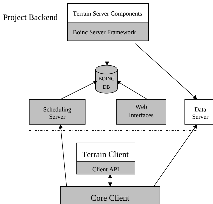
Figure 7 Components of Terrain@home project (Based on BOINC general project component)
