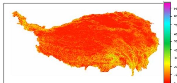
Figure10 GTOPO30 Slope of Tibet
