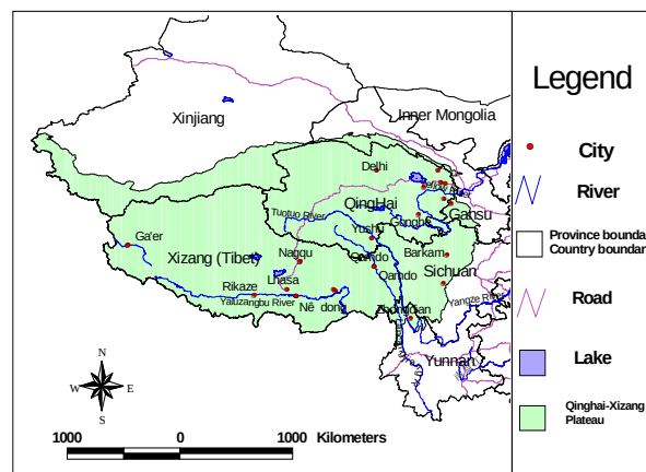
Figure 1. Shape of Tibet Plateau
