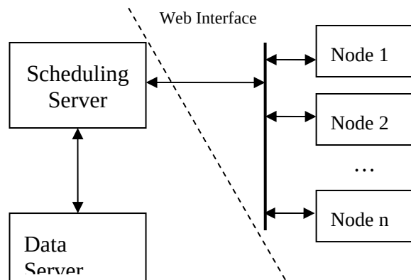
Figure 8 Terrain@home Architecture
