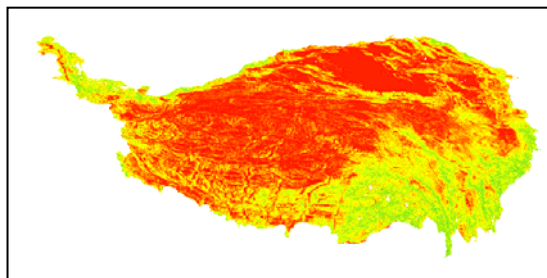
Figure9 SRTM3 Slope of Tibet
