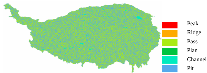
Figure11 Terrain Feature Map Grid
